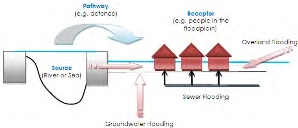
Figure 1-2: Source-Pathway-Receptor Model
