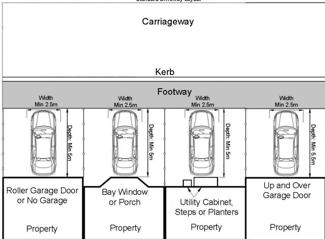
Appendix 2 Standard Driveway Layout
